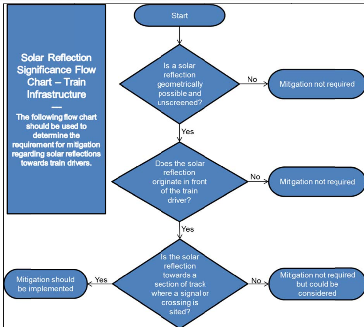
Figure 14 Train driver impact significance flow chart
