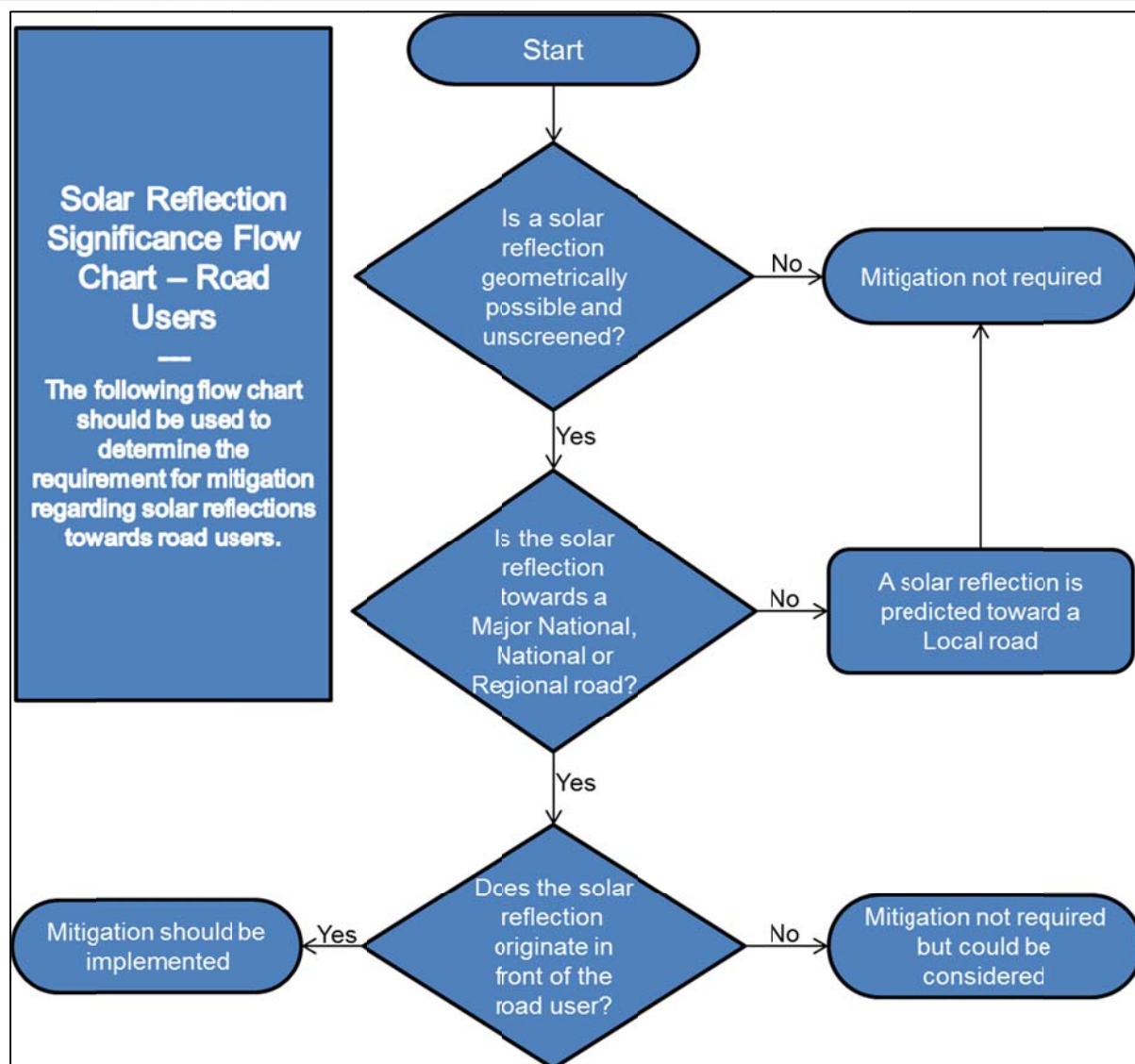
Figure 12 Road user impact significance flow chart
