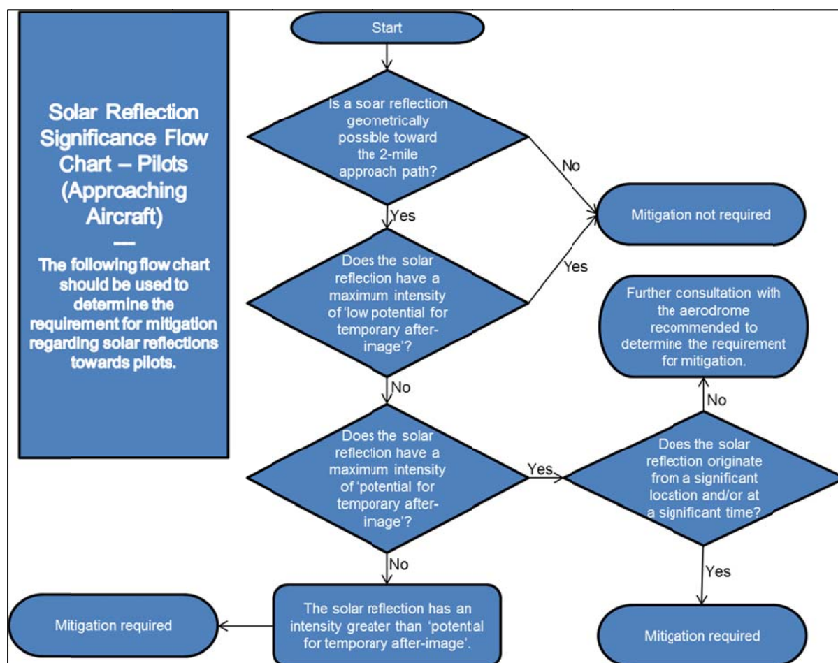
Figure 17 Pilots (approaching aircraft) impact significance flow chart
