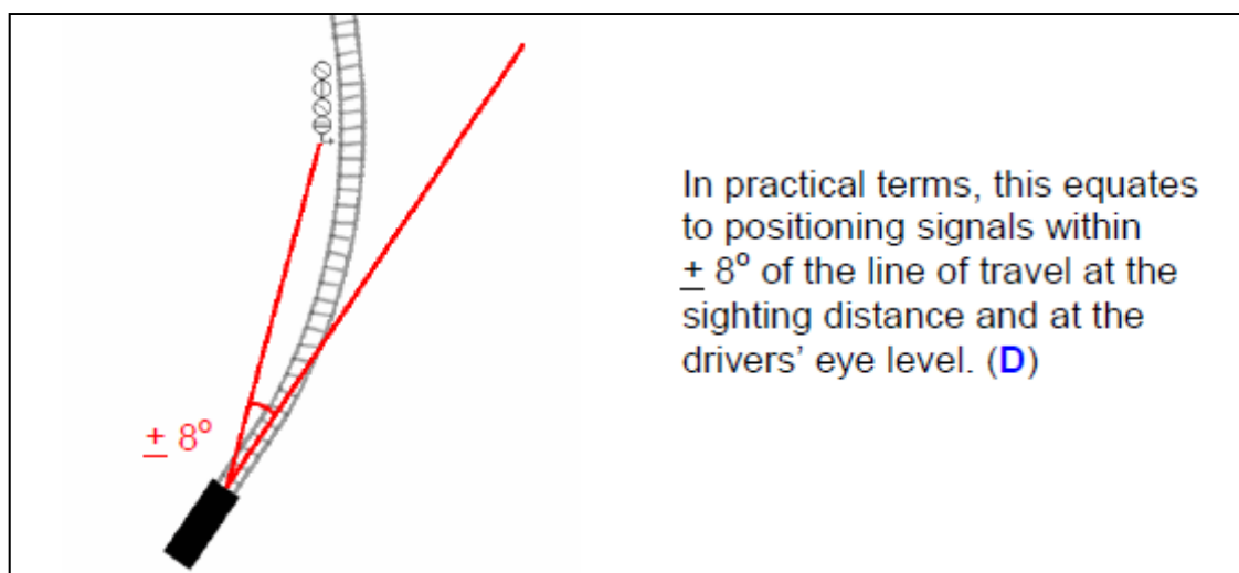
Figure 2 Signal positioning
