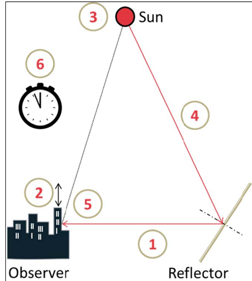
Figure 6 Conditions for determining significant glint and glare
