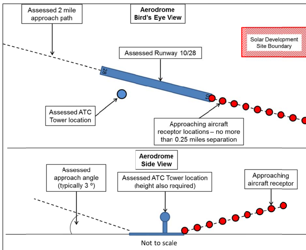
Figure 15 Illustration showing receptor identification process – aviation
